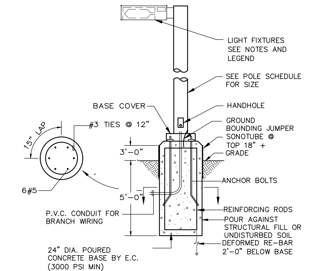
SITE LIGHT BASE DETAIL NOT TO SCALE NOTE: BUILDING PERMIT REQUIRED FOR LIGHT POLE FOUNDATIONS PRIOR TO INSTALLATION.
