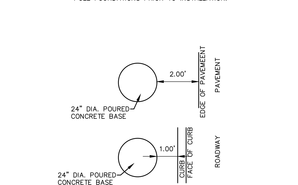
SITE LIGHT BASE PLACEMENT DETAIL NOT TO SCALE
